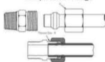
Compression Fittings
