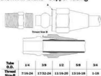
D.O.T. Air Brake - Copper Tubing
